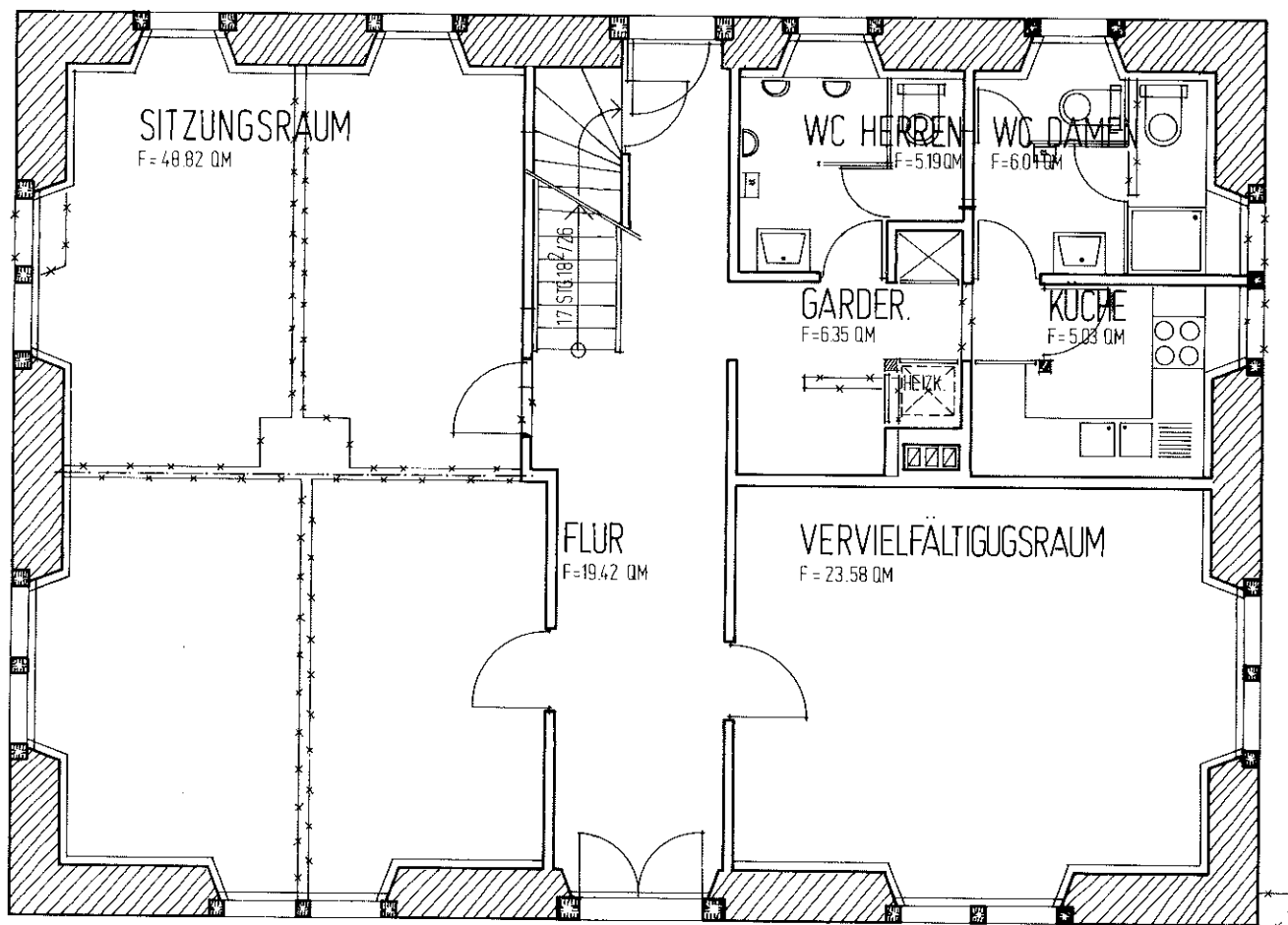
91 Grundriß Erdgeschoß
